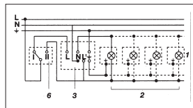
4. Connection to double-throw switch for permanent light and automatic operation
