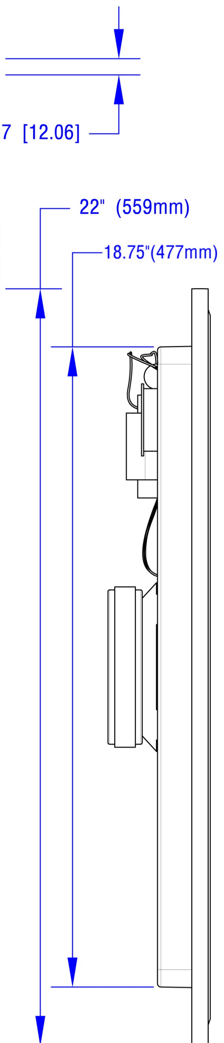
SIDE VIEW
