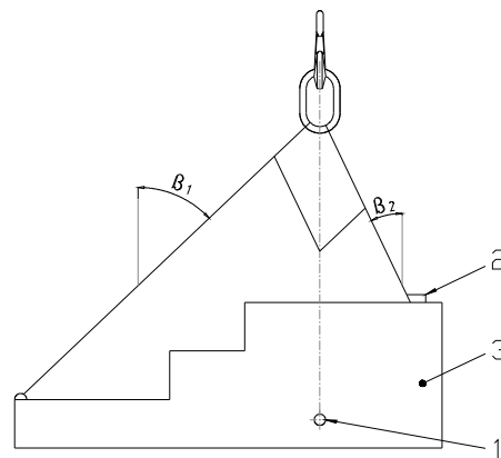
Fig. 2 (asymmetrical load)
